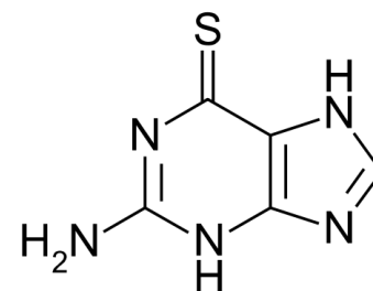
Thioguanine
