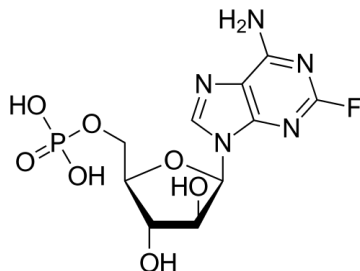
Fludarabine phosphate
