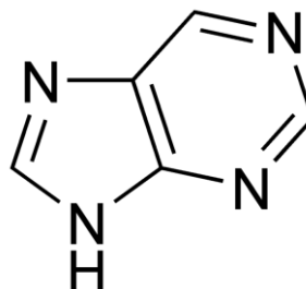
Purine
